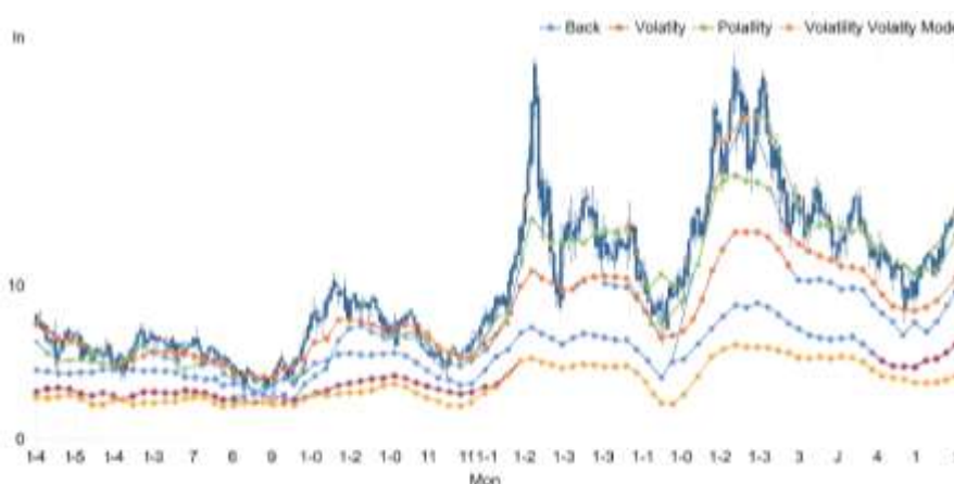
Fig. 2. Conditional stock return volatility (GARCH).
